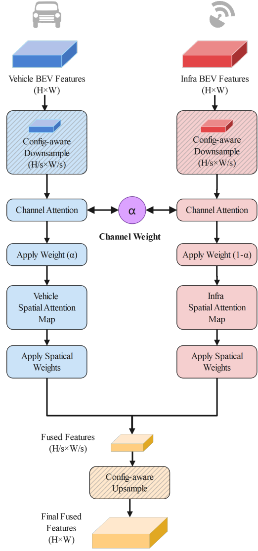
Fig. 3: Architecture of inter-node feature fusion combining Hierarchical Attention Fusion (HAF) and Adaptive Spatial Resolution (ASR) mechanisms. The shaded regions denote the ASR modules.
