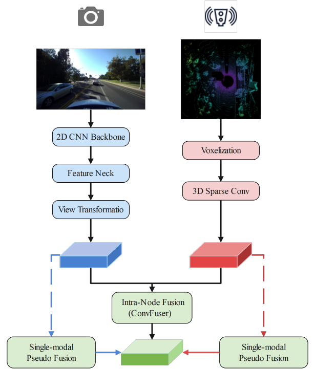
Fig. 2: BEV feature extraction process for heterogeneous sensors. Our framework handles various sensor configurations through specialized encoding paths for LiDAR and camera, along with intra-node fusion for multi-modal configurations and PseudoFusion for single-sensor scenarios.
