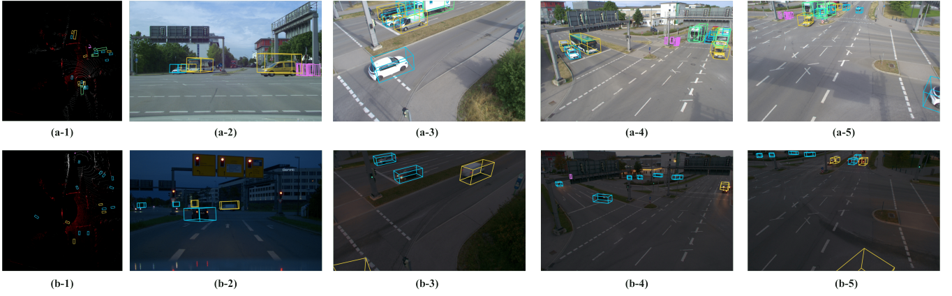
Fig. 4: Qualitative visualization of HeCoFuse detection results in the full sensor configuration (LC+LC) on the TUMTraF-V2X test set. The figure illustrates detection results in both daytime (first row) and nighttime (second row) conditions. (a-1, b-1) BEV perspective showing fused LiDAR point clouds with detection results from both vehicle and infrastructure; (a-2, b-2) vehicle-mounted camera view with corresponding 2D projections of 3D detections; (a-3, a-4, a-5, b-3, b-4, b-5) three different infrastructure camera views with projected detection results.
