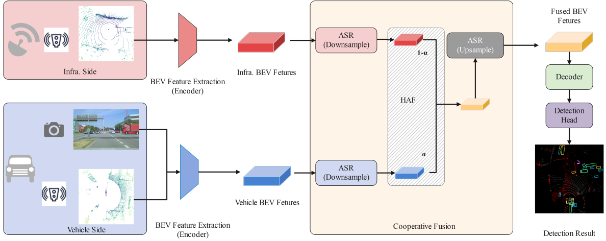
Fig. 1: HeCoFuse framework overview. Here, the LC+L case is used as an example (vehicle: LiDAR+Camera; infrastructure: LiDAR); for other vehicle–infrastructure sensor combinations, the per-node setups vary accordingly. The framework integrates features via Hierarchical Attention Fusion (HAF) and balances resolution through Adaptive Spatial Resolution (ASR) across different scenarios.
